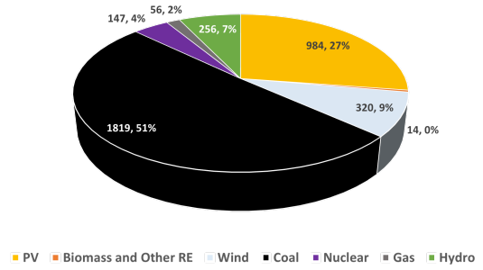
Source wise projected gross generation (BU) in 2035-36
